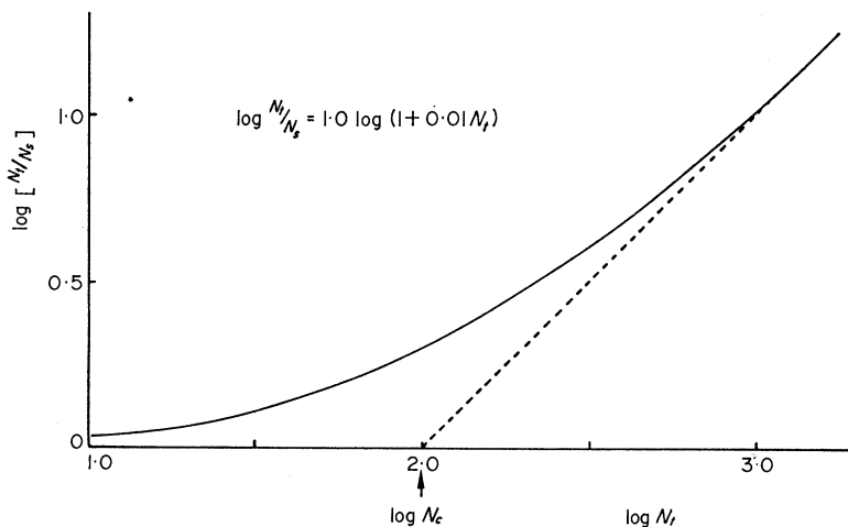
FIG. 3. A density-dependent relationship from equation (11) where a = 0.01 and b = 1.0 .
