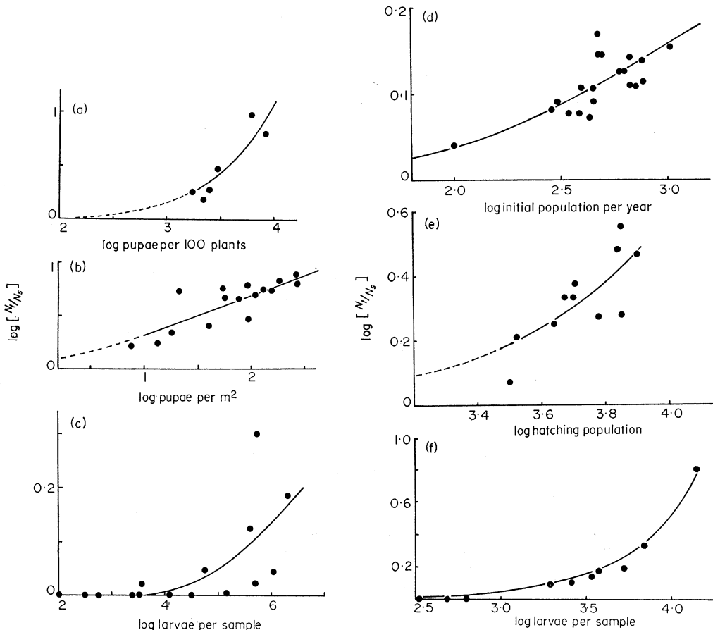
FIG. 8. Density-dependent relationships from field data and their description based on equation (12). (a) Cabbage root fly ( Erioischia brassicae (Bouché)) pupal mortality. a = 0.00011 , b = 3.16 (data from Benson 1973). (b) Winter moth ( Operophtera brumata (L.)) pupal mortality. a = 0.6 , b = 0.38 (data from Varley & Gradwell 1968). (c) Larch tortrix ( Zeiraphera diniana Gn.) larval disease. a = 0.000018 , b = 0.11 (data from Varley & Gradwell 1970, after Auer 1968). (d) Clutch size reduction in the great tit ( Parus major L.) plotted against log maximum clutch size ( \log N_t ). a = 0.0064 , b = 0.18 (after Krebs 1970). (e) Chick mortality in the partridge ( Perdix perdix L.) plotted against log hatching population ( \log N_t ). a < 0.000005 , b > 28.58 (after Blank et al. 1967). (f) Larval starvation in the Colorado potato beetle ( Leptinotarsa decemlineata (Say)) plotted against log larval density ( \log N_t ). a = 0.00007 , b = 30.95 (data from Harcourt 1971).
