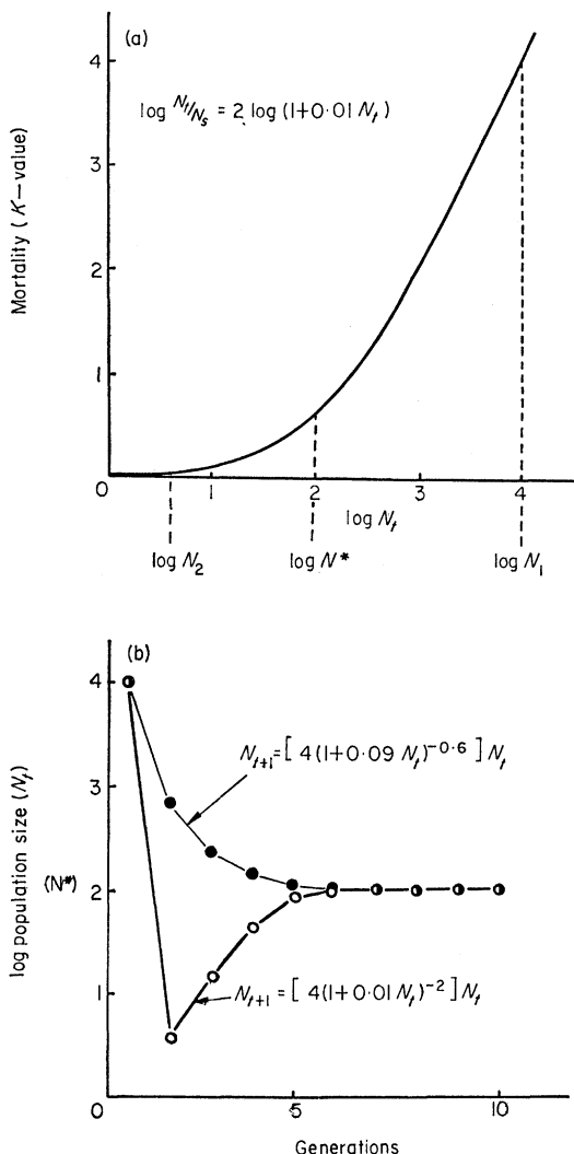
FIG. 9. (a) Density-dependent relationship calculated from equation (12) where mortality (expressed as a k -value) is plotted against \log population density ( \log N_t ). See text for further explanation. (b) Population changes calculated from eqn. (11) following displacement from the equilibrium ( N^* = 100 ). \circ : a = 0.01 , b = 2 and \lambda = 4 (as in Fig. 9a). Overshooting when displaced above N^* as shown; exponential damping when displaced below. \bullet : a = 0.09 , b = 0.6 and \lambda = 4 . Exponential damping when displaced above or below N^* .
