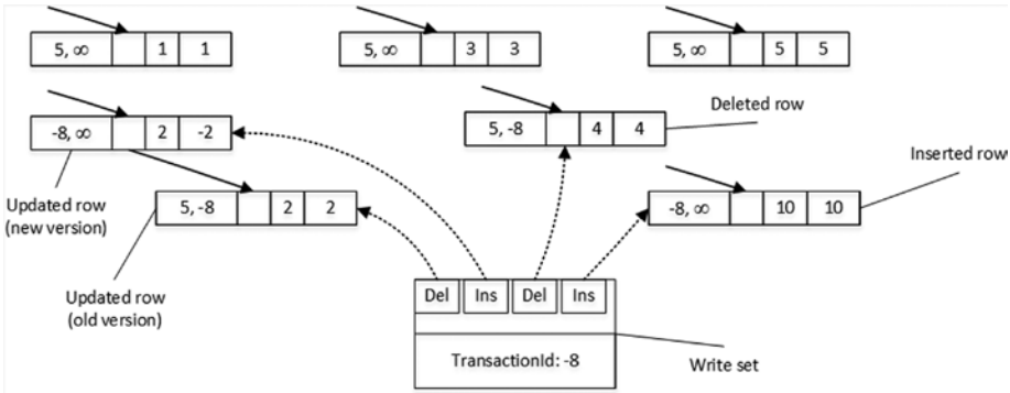
Figure 7-3. Data in the dbo.HKData table after modifications
