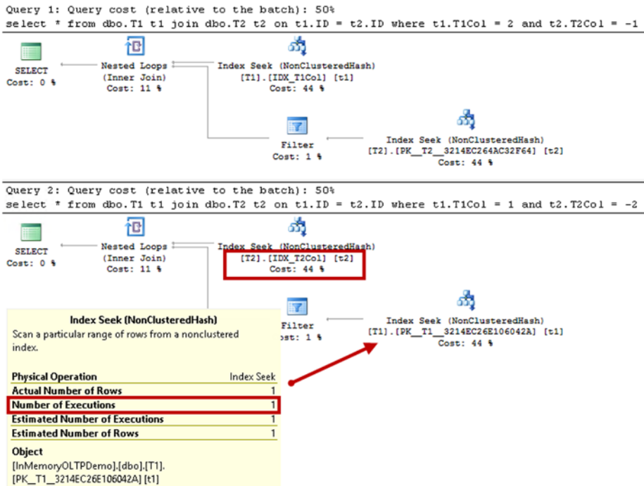
Figure 4-13. Missing statistics and inefficient execution plans: execution plans after statistics update
