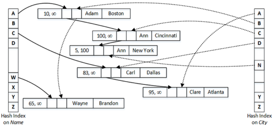
Figure 3-4. Data in the table after update
