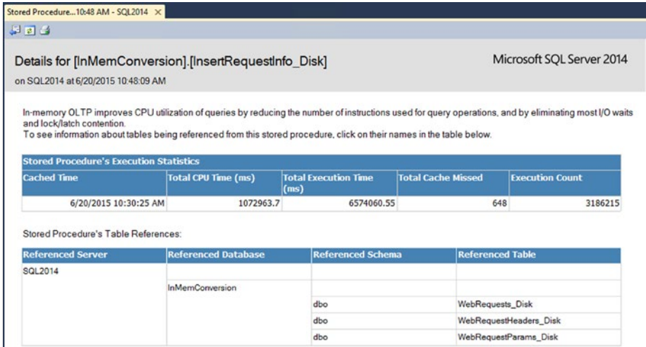
Figure D-13. Procedure-Level Statistics
