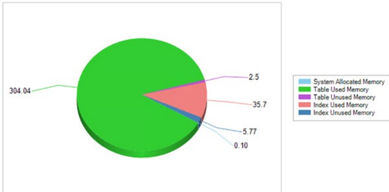
Memory Usage Details for Memory Optimized Tables (MB)
