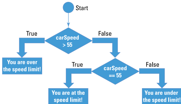
Figure 13-1: An if-else statement with an elsif.
