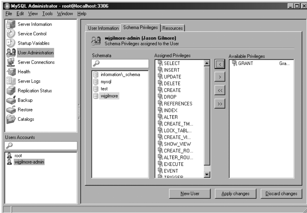
Figure 27-1. Managing user privileges with MySQL Administrator
