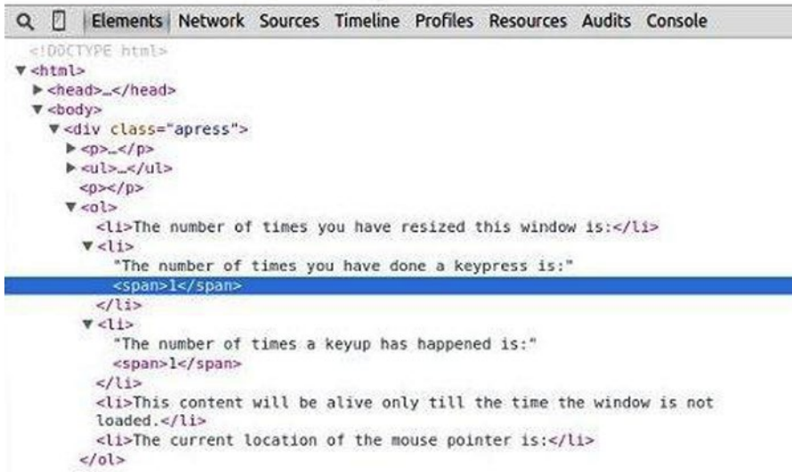
Figure 5-7. Count for single keypress and keyup events
