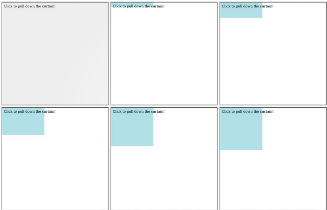
Figure 7-12. This sequence of frames shows how the mentioned sliding down animation takes place
