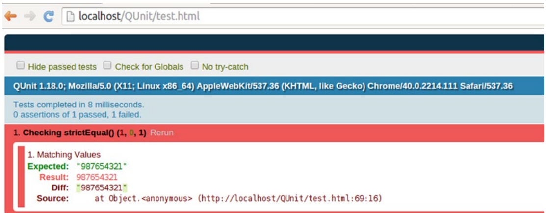
Figure 12-3. Output of strictEqual
