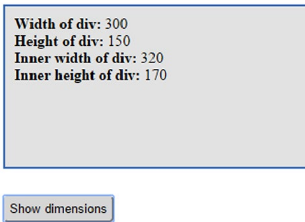
Figure 4-6. The width, height, inner width, and inner height of an element on a click event
