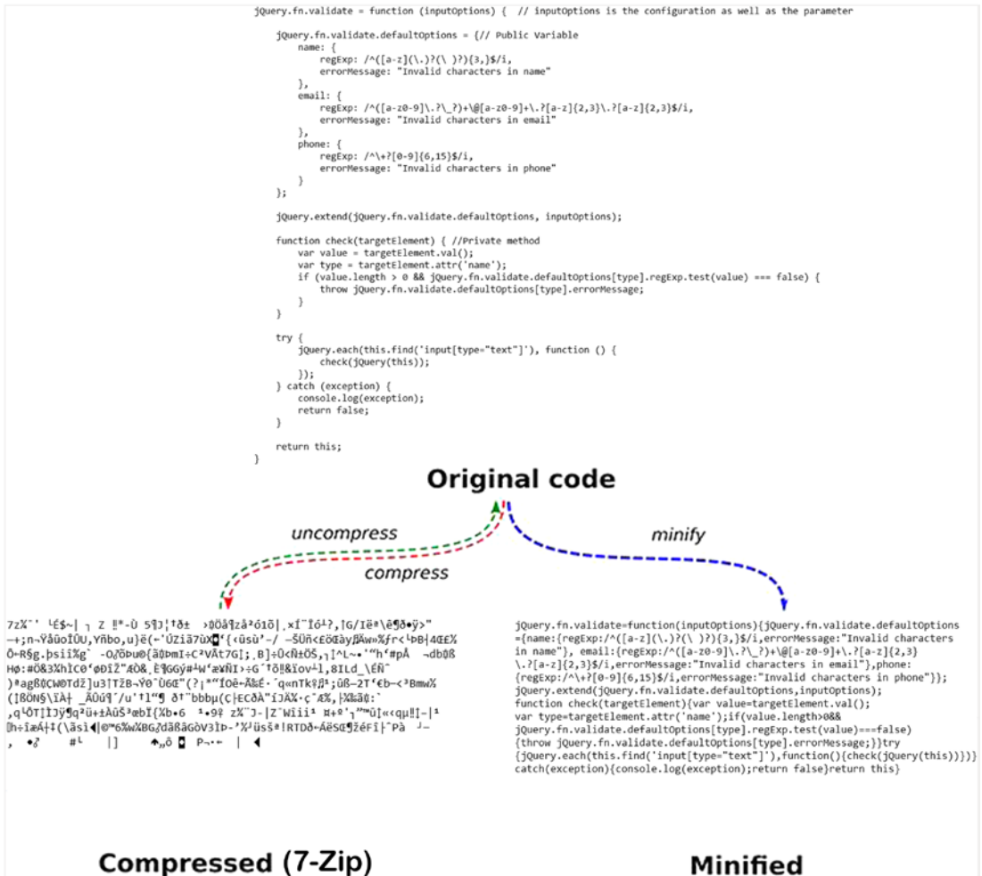
Figure 10-1. The difference between compression and minification
