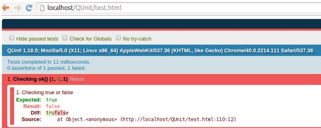
Figure 12-6. Execution of ok assertion
