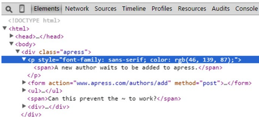
Figure 3-21. The effect of .has()
