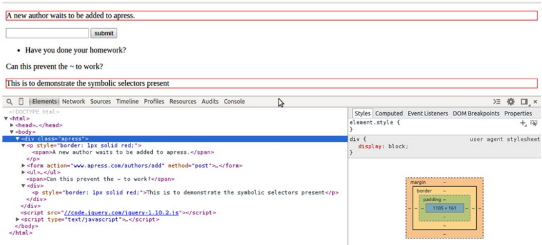
Figure 3-9. The found elements with borders
