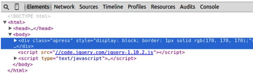
Figure 3-16. The output of .filter()
