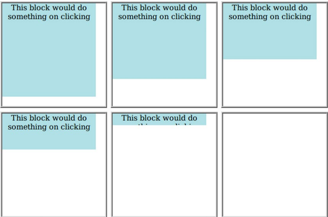
Figure 7-10. This shows the linear sliding up animation as a sequence of frames
