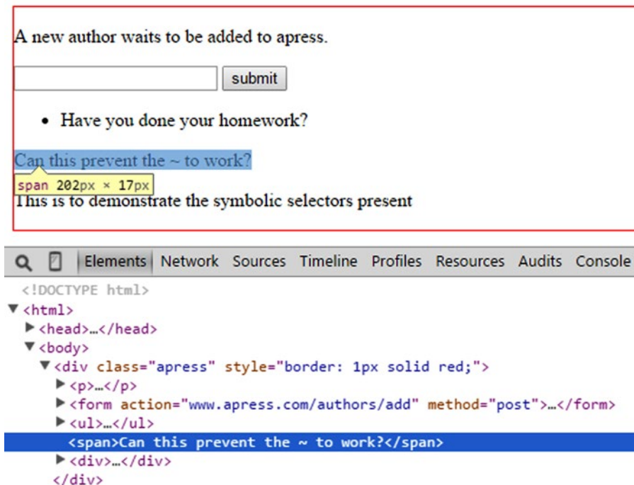
Figure 3-6. The result of the closest() method
