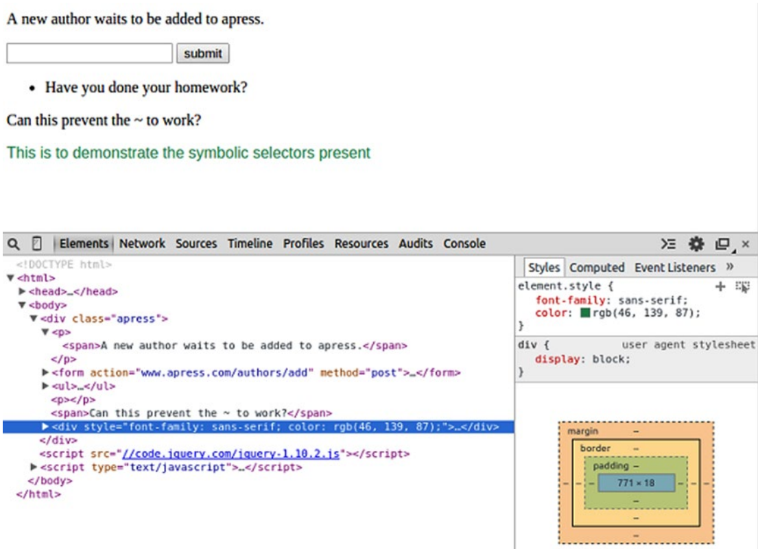
Figure 3-23. The output of the .not() method
