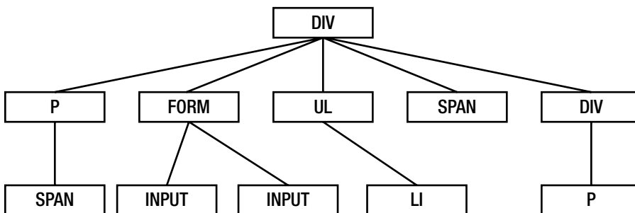
Figure 3-1. The DOM structure and hierarchy
