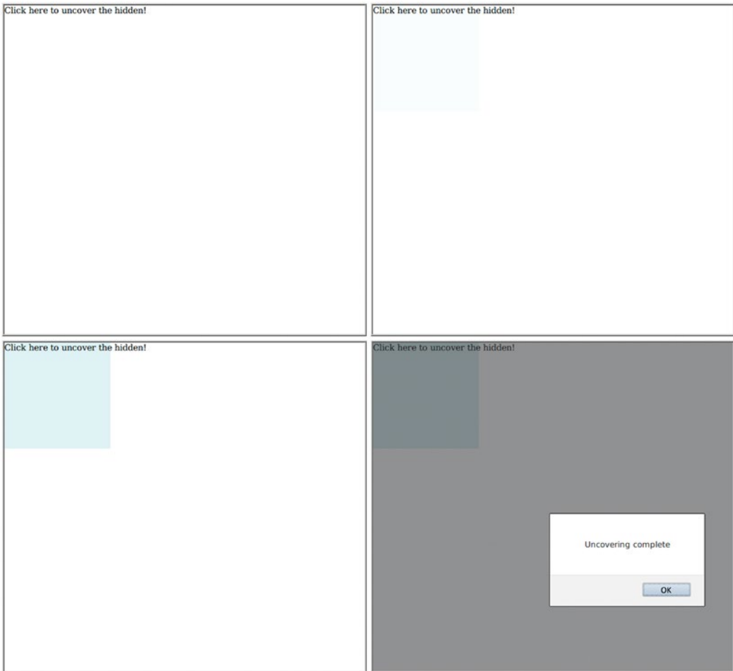
Figure 7-8. This frame sequence shows the same effect using the callback method
