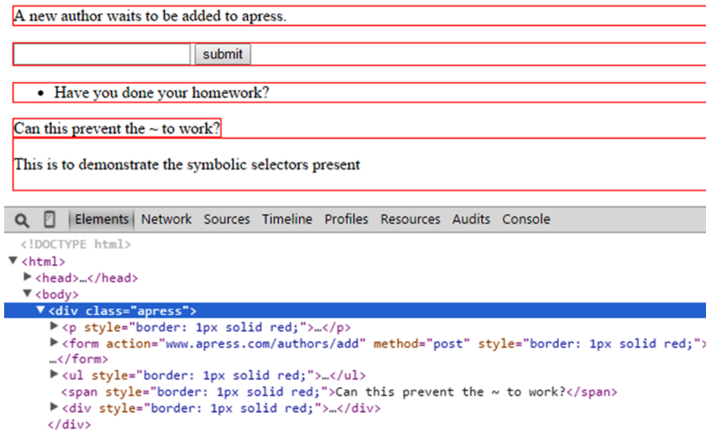
Figure 3-8. The result of the children() method
