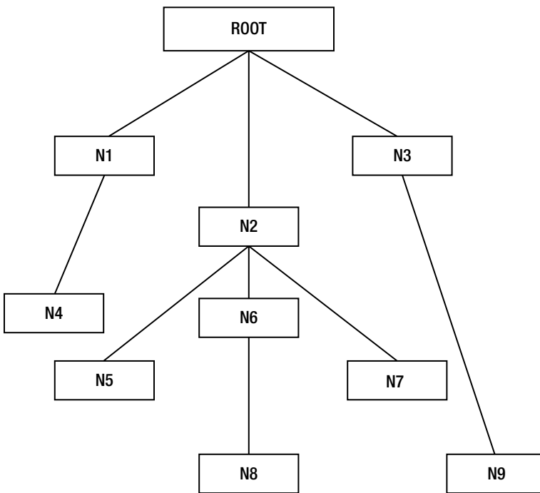
Figure 1-1. A drawing of the document object tree
