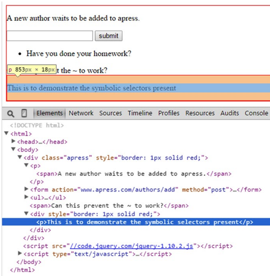
Figure 3-2. The immediate parent and an uneven border
