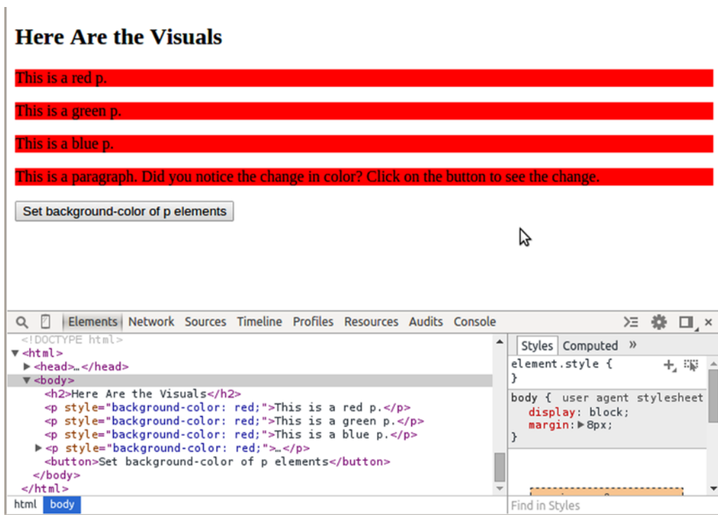
Figure 4-1. Code output with the property changed for all p elements
