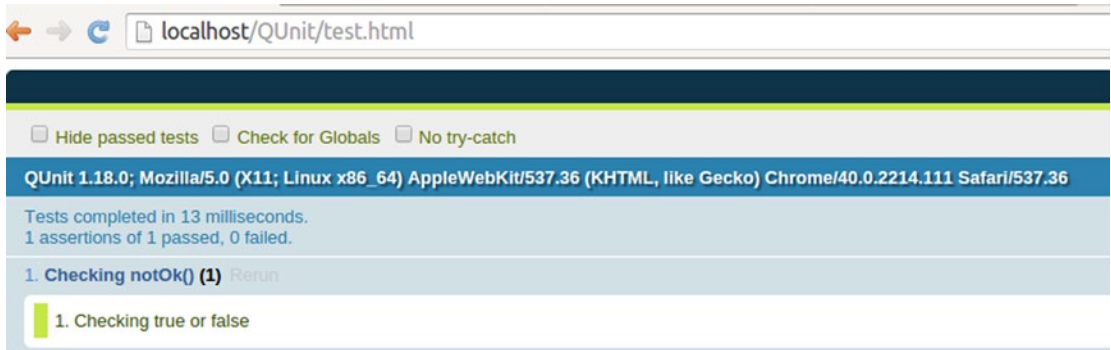
Figure 12-7. Output of test execution notOk
