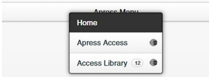
Figure 11-7. Code execution
