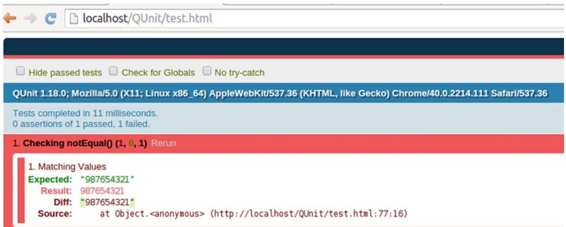
Figure 12-4. The notEqual assertion output
