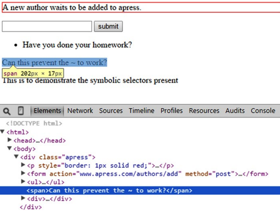
Figure 3-7. The styling result of our sample use of the closest() method
