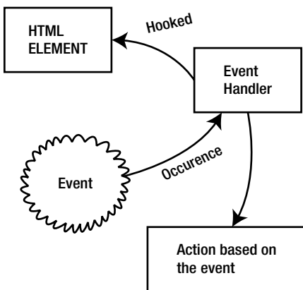
Figure 5-1. Illustration showing how events take place
