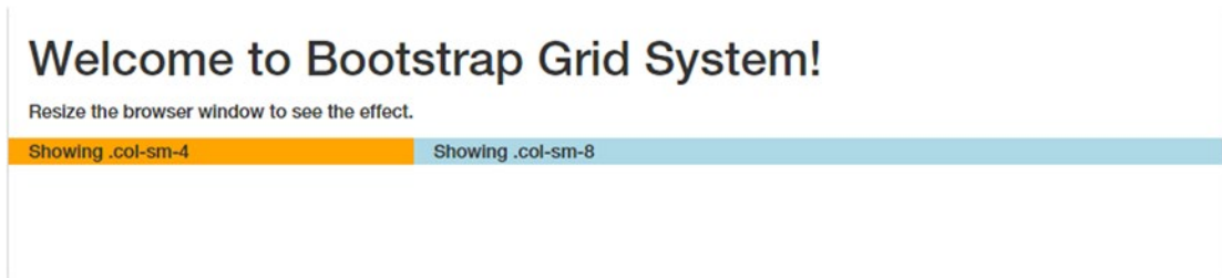
Figure 11-1. Output of our sample grid, with unequal column widths
