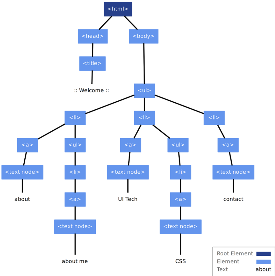
Figure 2-1. The DOM tree
