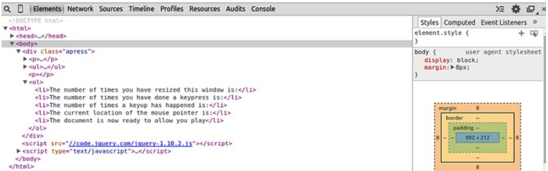
Figure 5-6. The output of the window load event
