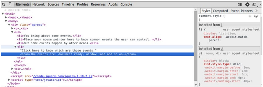
Figure 5-5. Showing mouse click event
