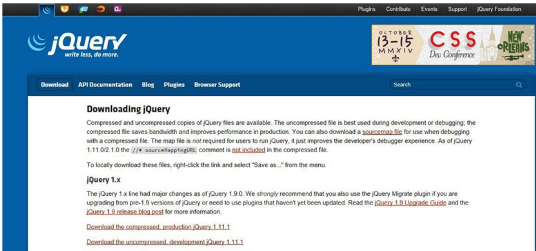
Figure 2-2. Downloading jQuery
