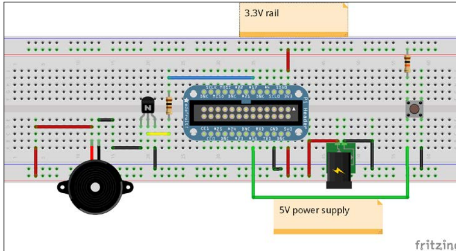
A buzzer and switch schematic created using Fritzing
